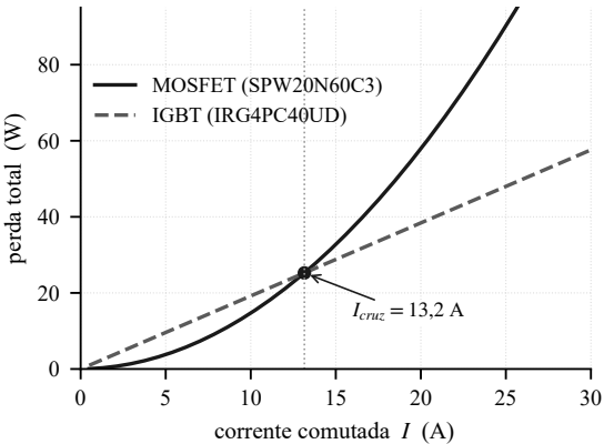
(a) V = 400\text{ V} , f_s = 20\text{ kHz}
